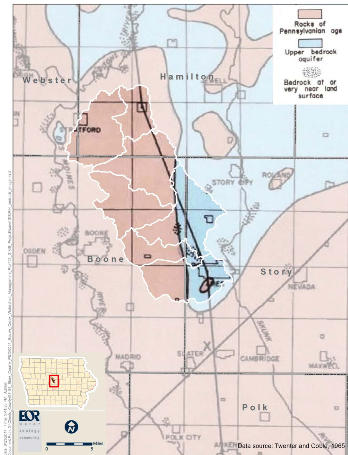
Figure 2-16. Uppermost Bedrock
